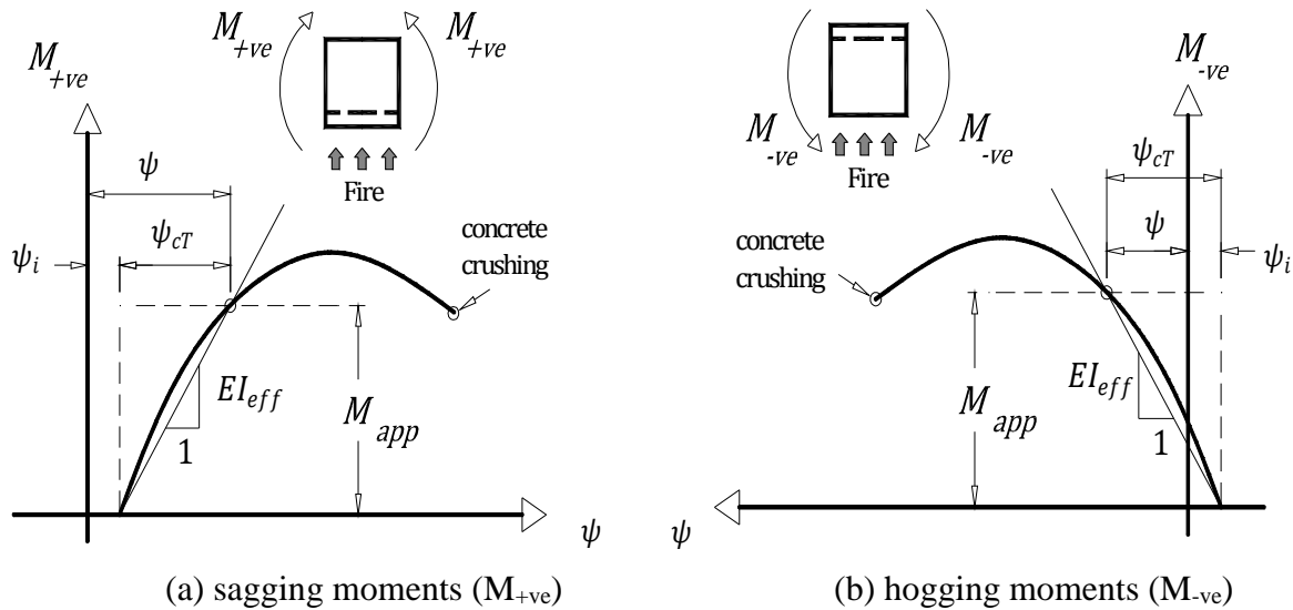
Fig. 2 (M)-(\psi) diagrams for RC sections during fire
