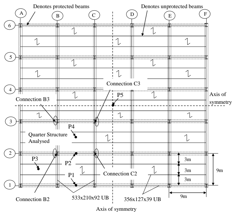
Fig. 1 Layout of 45m x 45m composite floor
